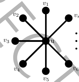
Figure 1: Star graph S_n
