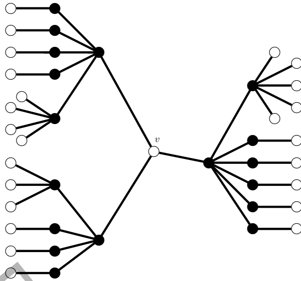
Figure 2: Graph G with \gamma_{st}(G) = 18 and \gamma_{st}(G - v) = 15 .
