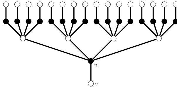
Figure 5: Graph G with \gamma_{st}(G) = 17 and \gamma_{st}(G/v) = 20 .
