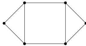
Figure 1: A non-chordal graph G with \text{reg}(J_G) \leq 5
